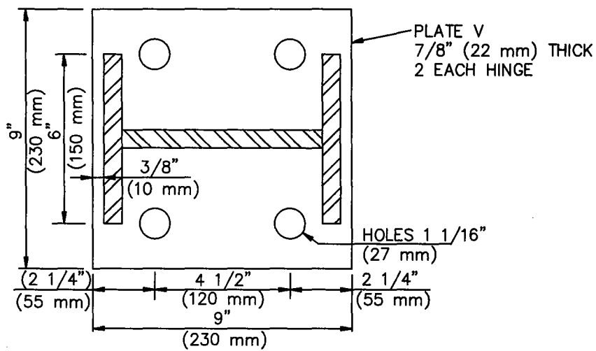
SECTION T-T
