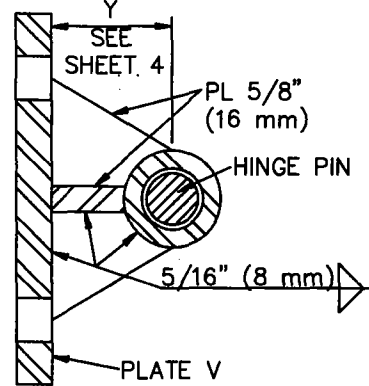
SECTION T-T
