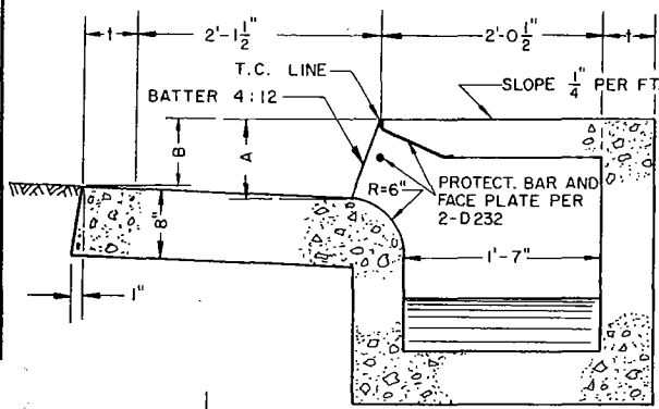
SECTION F-F A = C.F. PLUS 1" FOR 8" C.F.: B = 5 3/4" FOR 6" C.F.: B = 3 3/4"
