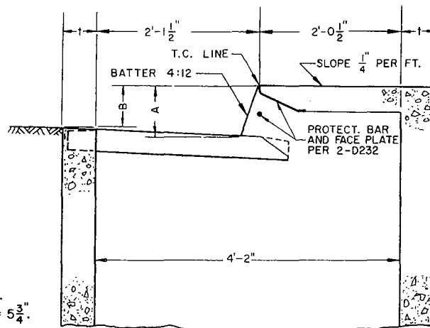
SECTION G-G
