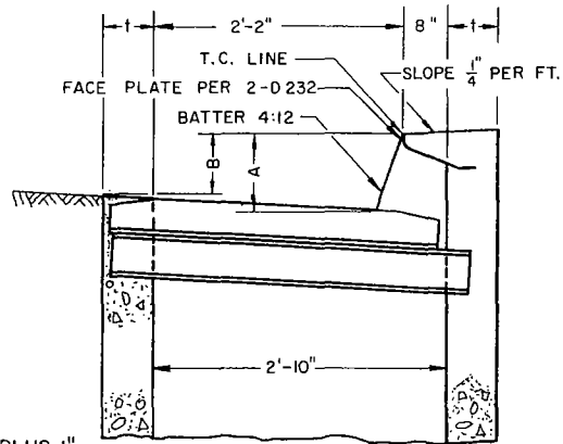
A = C.F. PLUS 1" FOR 8" C.F.: B = 5 3/4" FOR 6" C.F.: B = 3 3/4"
