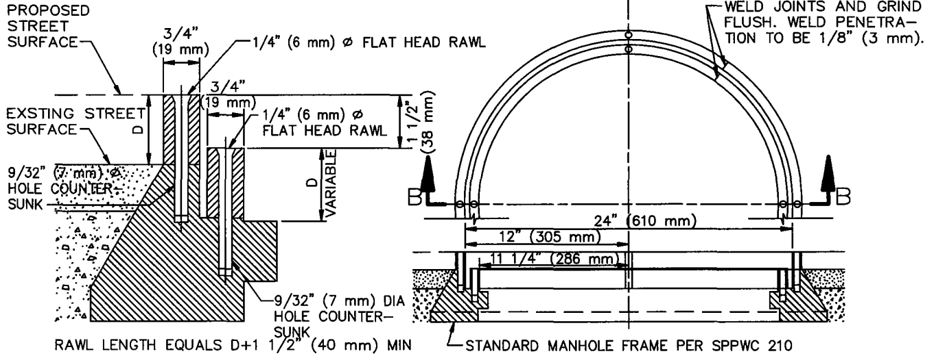
SECTION B-B
