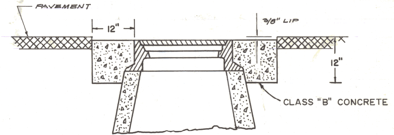
CROSS SECTION
