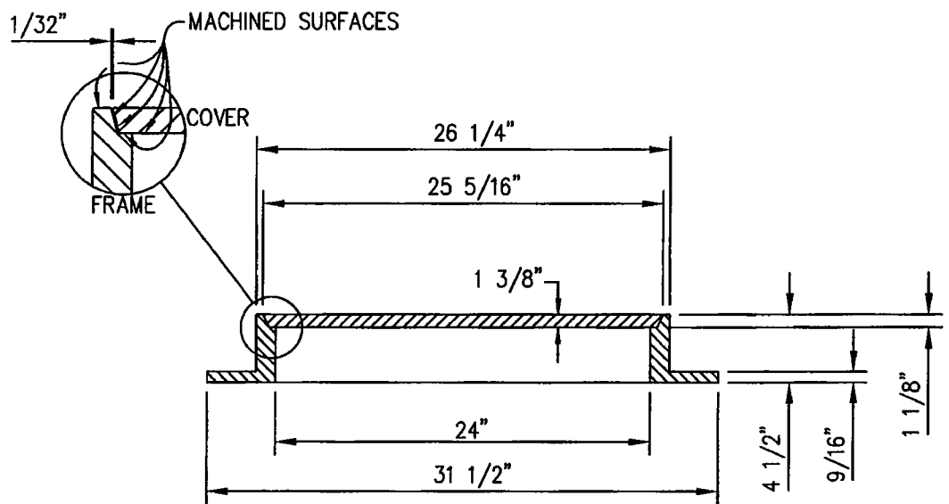
SECTION A-A TYPICAL FRAME AND COVER DETAIL
