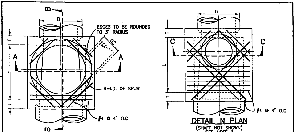
PLAN (SHAFT NOT SHOWN)
