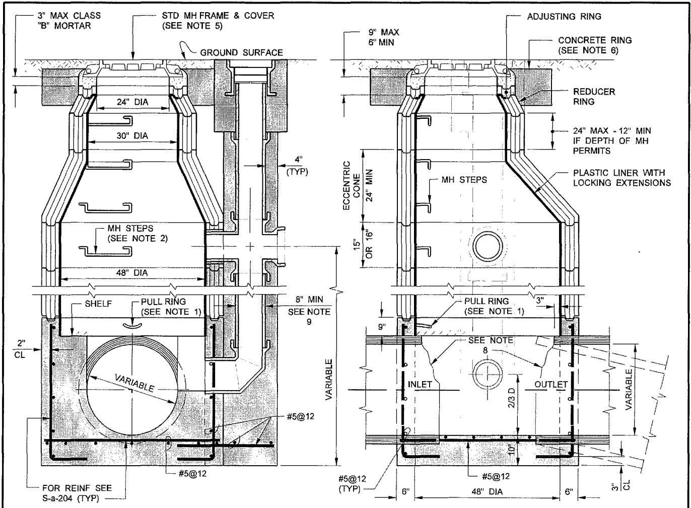
SECTION B-B
