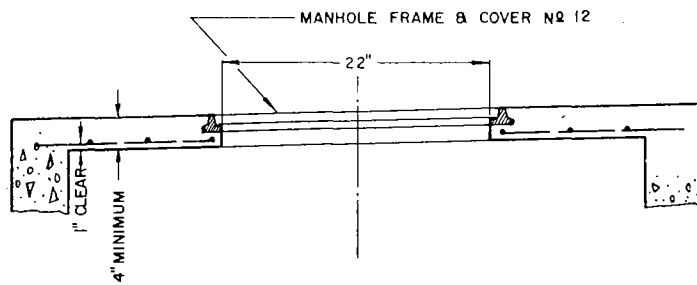
DETAIL OF STEEL REINFORCING FOR M.H. FRAME & COVER NO 12
