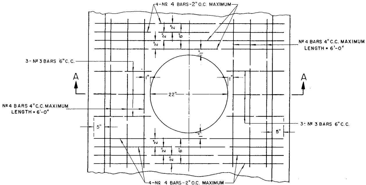
DETAIL OF STEEL REINFORCING FOR M.H. FRAME & COVER NO 12
