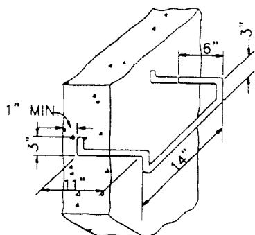
STEP DETAIL
