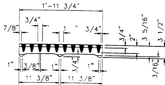
SECTION A-A CAST NODULAR IRON GRATE
