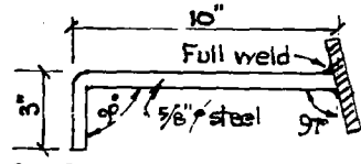
DETAIL OF ANCHOR 3'-6" C.C. for 7' Basin 2'-6" C.C. for 10' Basin
