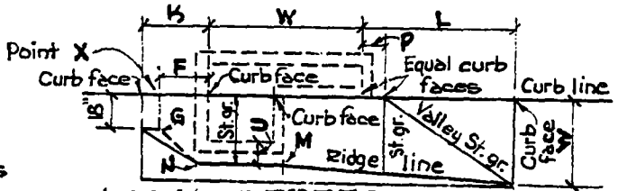
LOCAL DEPRESSION DETAIL
