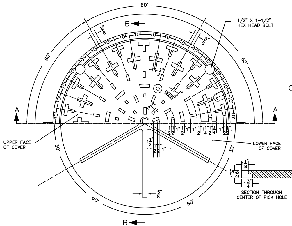
HALF PLAN OF HEAD AND COVER
