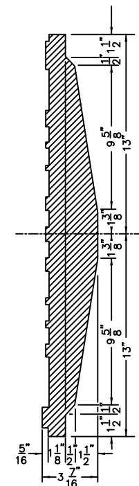
SECTION B-B
