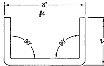
DOWEL DETAIL
