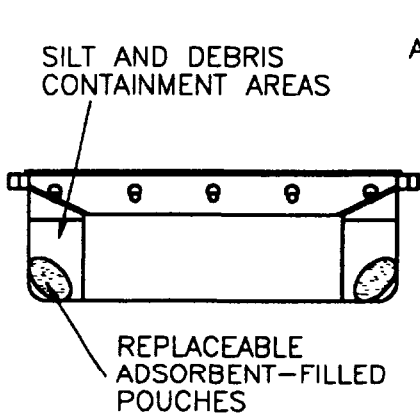
SECTION VIEW
