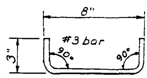
DETAIL OF DOWEL
