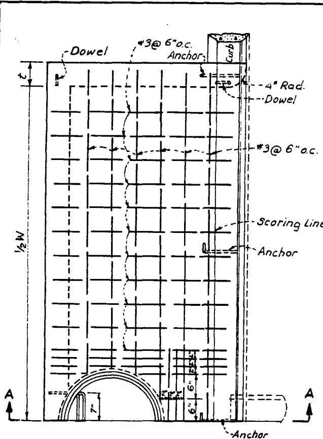
HALF PLAN SYMMETRICAL ABOUT A-A
