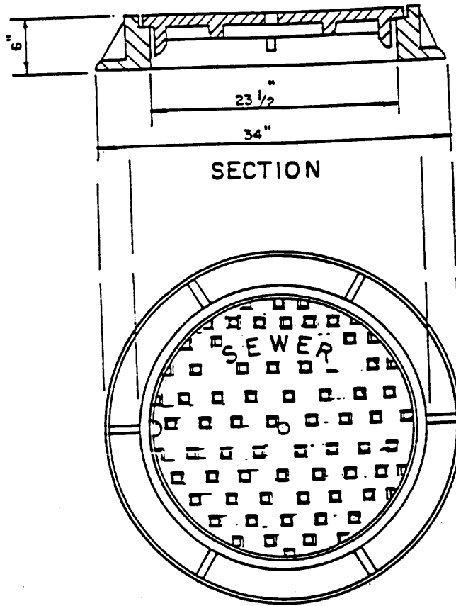
PLAN
