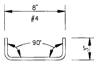
DOWEL DETAIL
