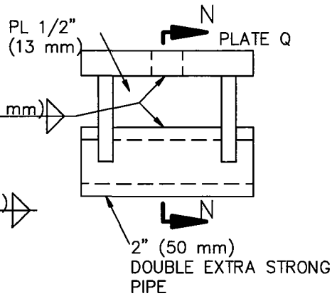
DETAIL M
