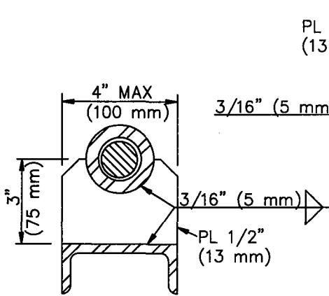
SECTION L-L
