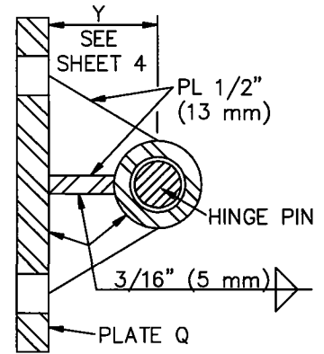
SECTION N-N
