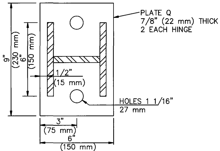
DETAIL P
