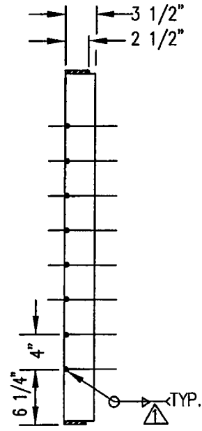
SECTION C-C
