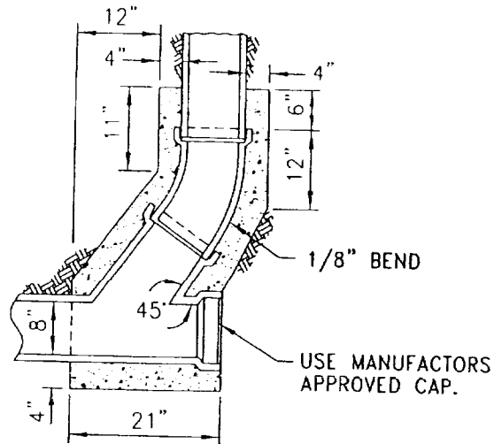
SECTIONAL ELEVATION
