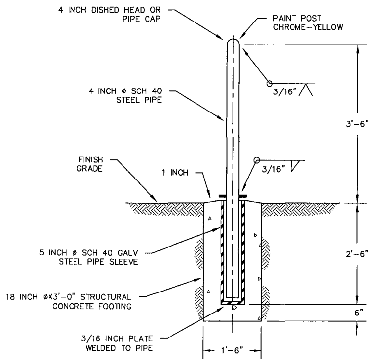
REMOVABLE BOLLARD DETAIL
