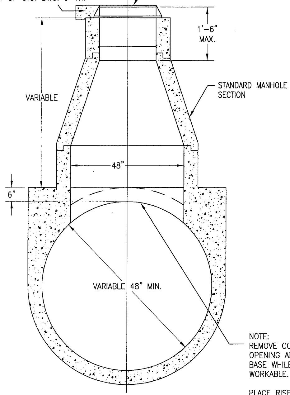
TYPE A CAST-IN-PLACE PIPE ONLY
