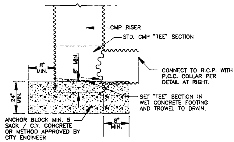
CONNECTION AND RISER DETAIL
