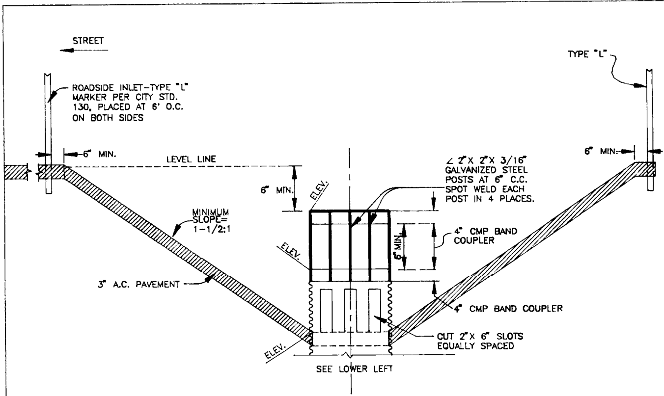
INLET DETAIL
