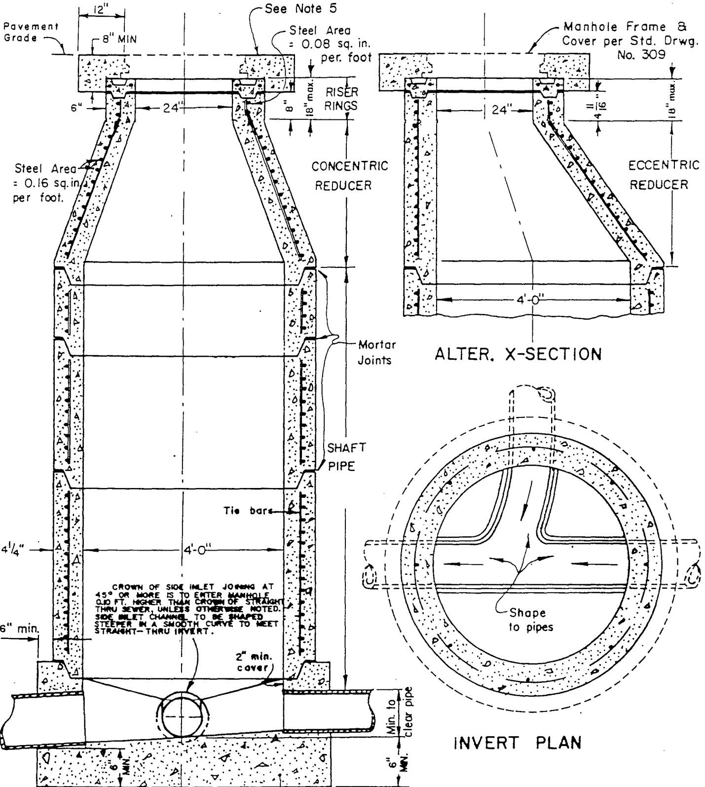
X-SECTION
