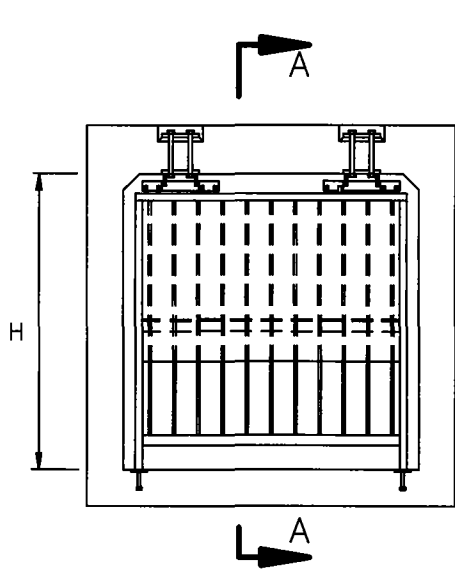
TWO-HINGED INLET/OUTLET BARRIER FOR RCB
