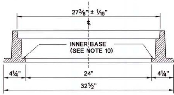
SECTION THRU FRAME
