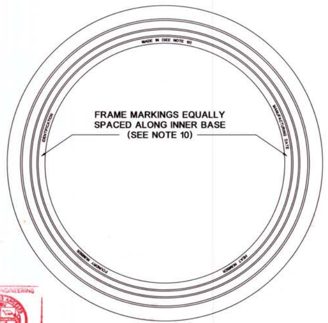
PLAN - TOP OF FRAME
