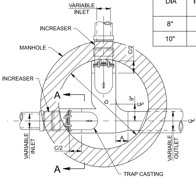
PLAN - DOUBLE TRAP BASE
