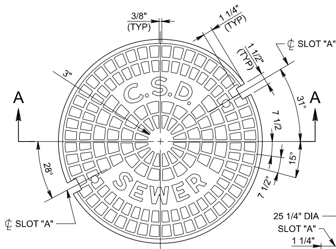
PLAN OF COVER TOP VIEW
