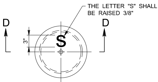
ACCESS COVER
