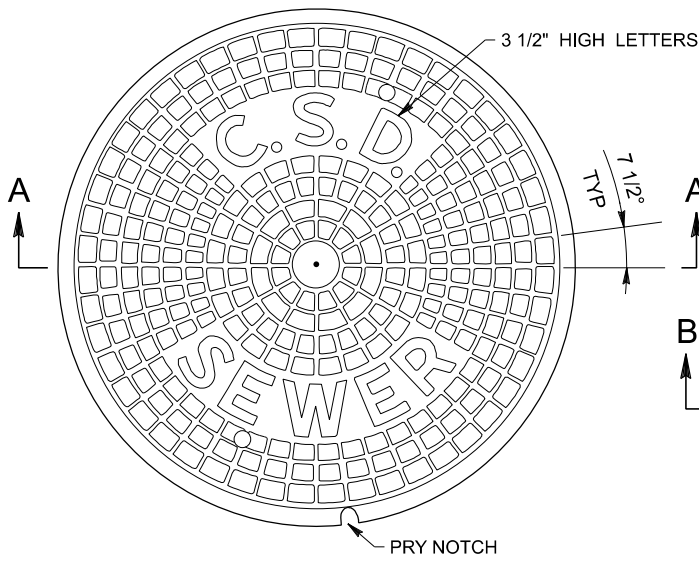
PLAN OF COVER TOP VIEW
