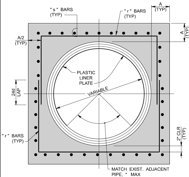
CROSS SECTION
