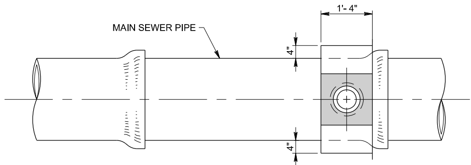
PLAN-SECTION B-B
