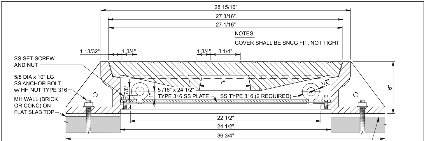
SECTION MANHOLE FRAME AND COVER
