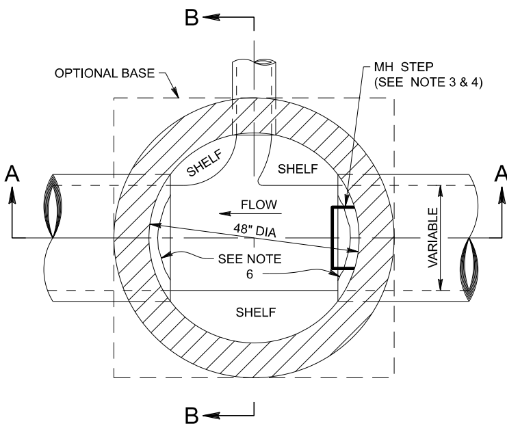
PLAN SECTION C-C
