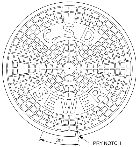
PLAN OF COVER
