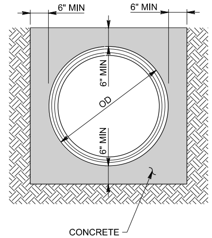
CONCRETE ENCASEMENT LOAD FACTOR = 4.5)
