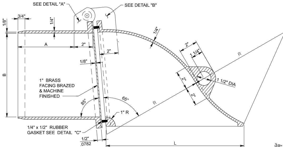
SECTIONAL VIEW
