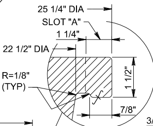
PLAN OF COVER TOP VIEW
