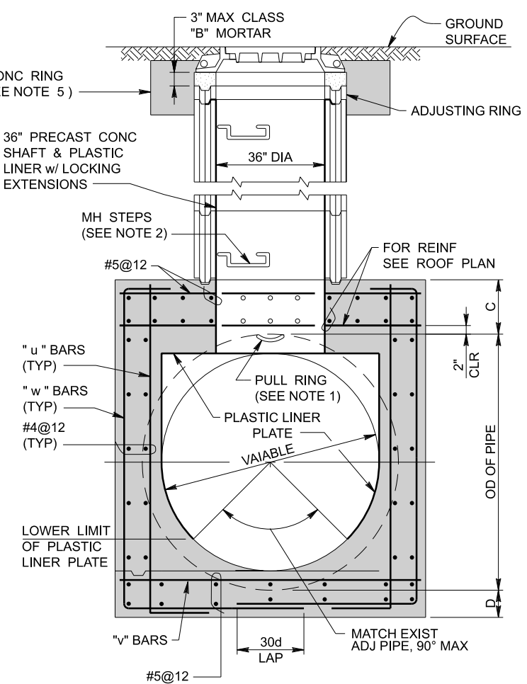
CROSS SECTION
