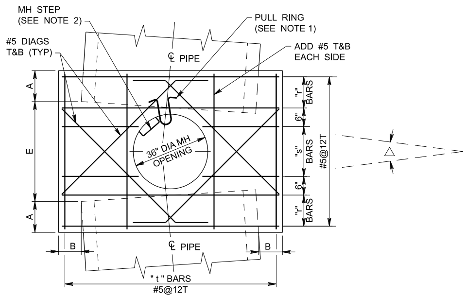
ROOF PLAN 0° TO 15° FOR 48" TO 96" PIPE
