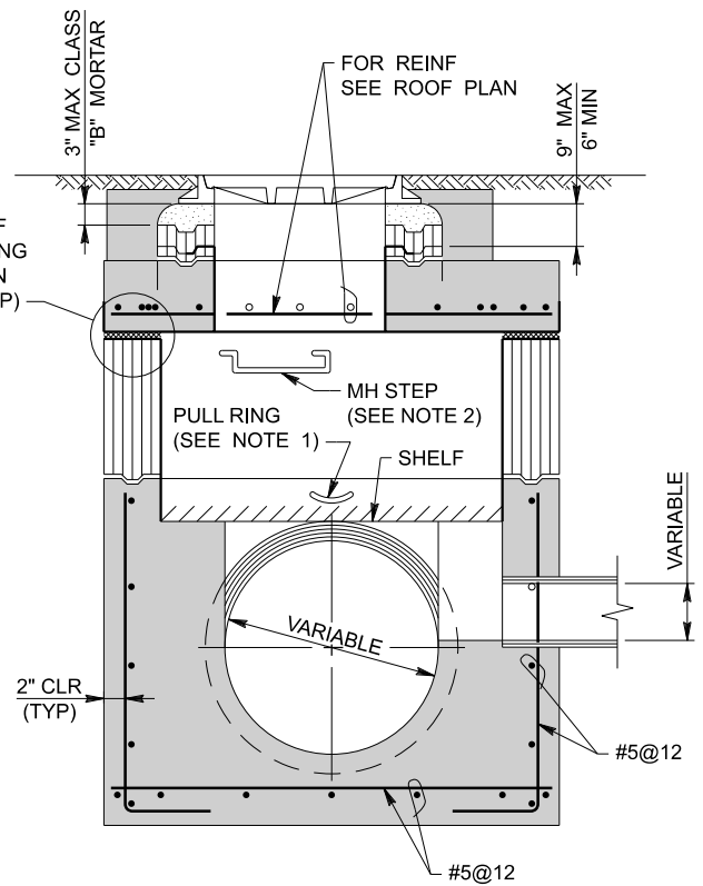
SECTION B-B
