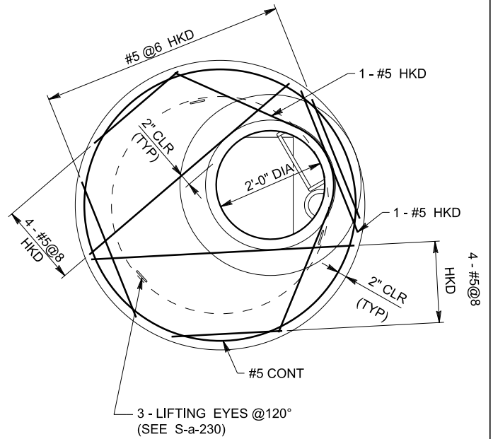
ROOF PLAN
