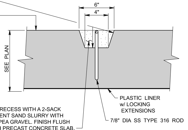
SECTION B-B
