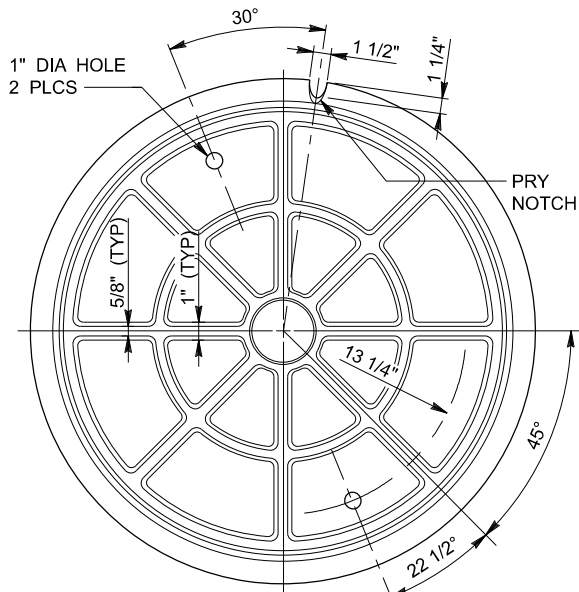
PLAN OF COVER
