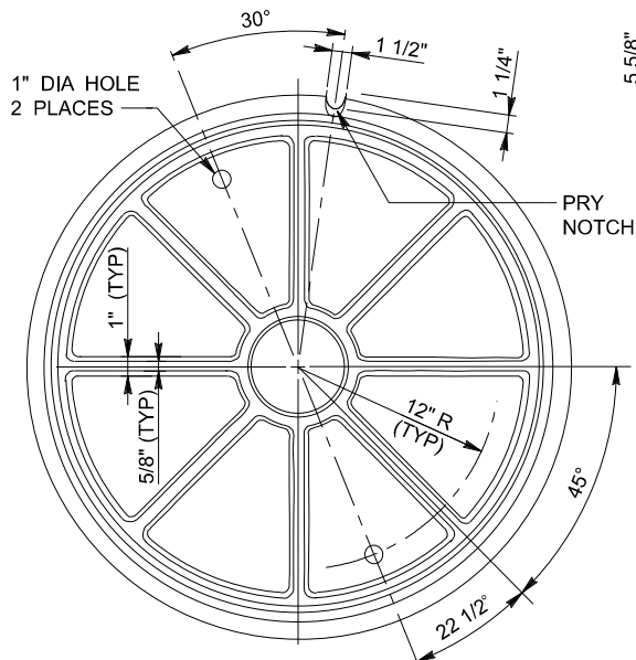
PLAN OF COVER BOTTOM VIEW
