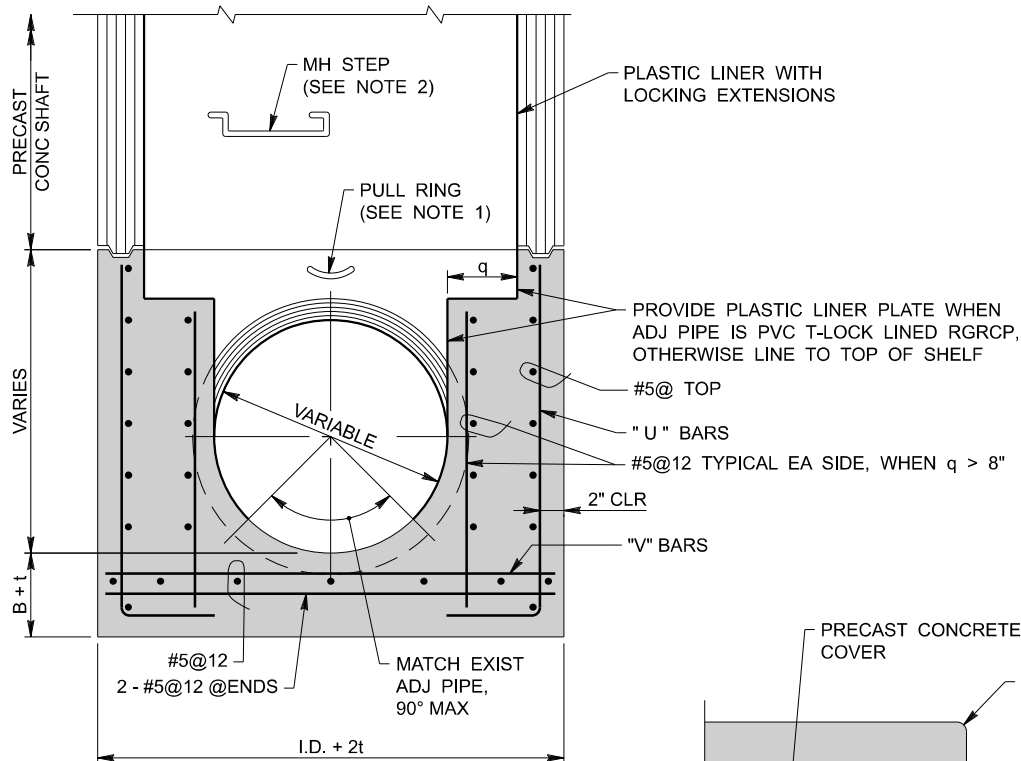
SECTION C-C
