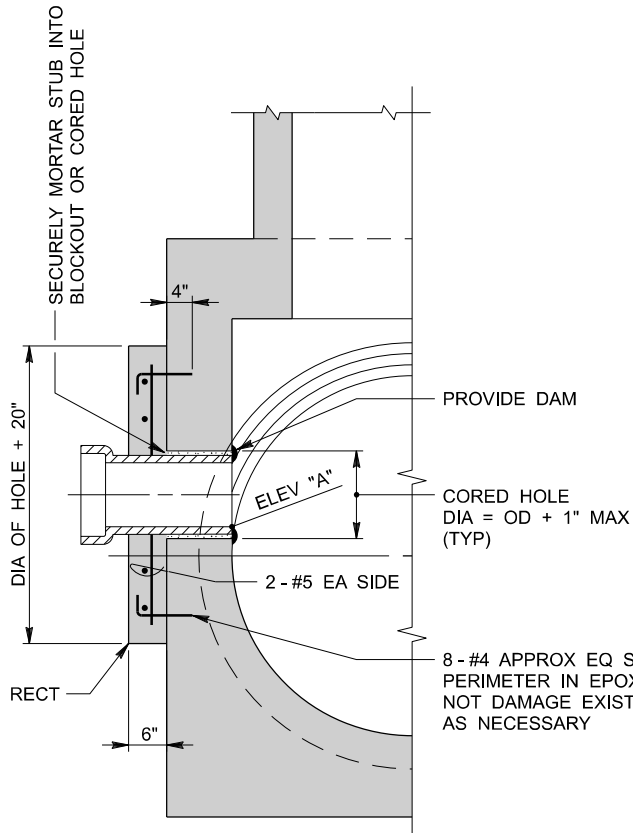
CONNECTION TO REINFORCED CONCRETE STRUCTURE
