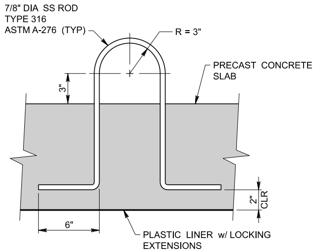
TYPE I LIFTING EYE
