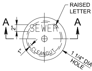
ACCESS COVER
