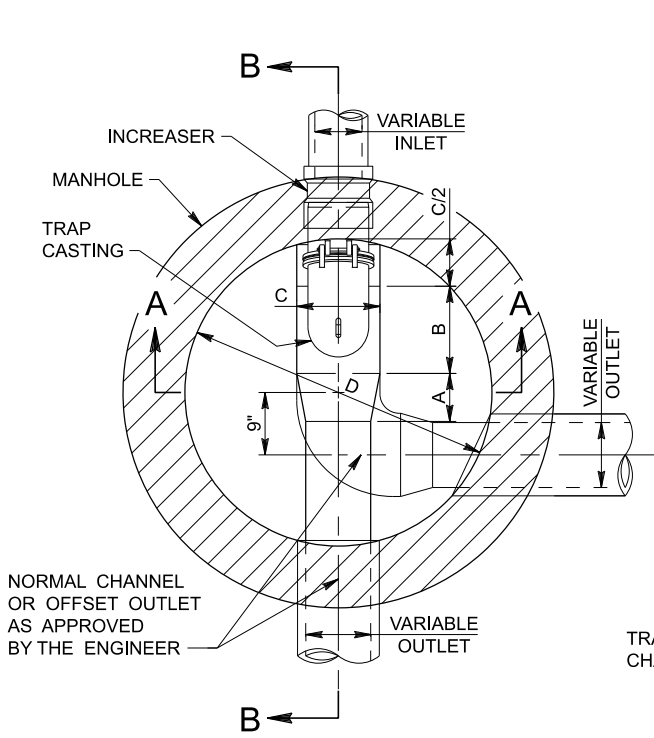
PLAN - SINGLE TRAP BASE
