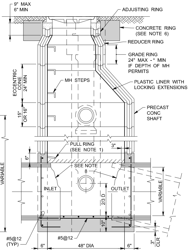
SECTION B-B
