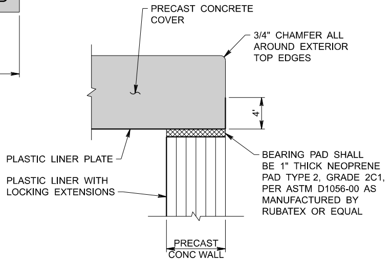
ROOF EDGE SEALING DETAIL
