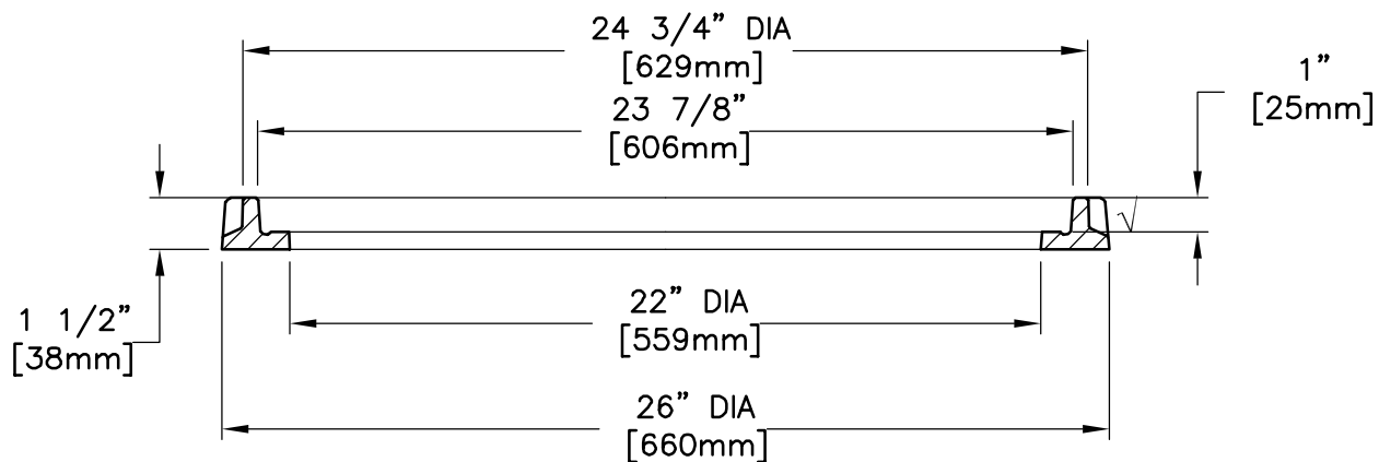
FRAME SECTION
