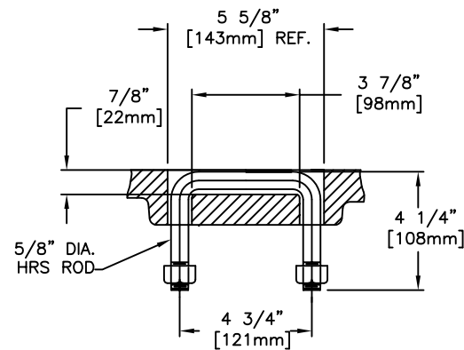
HANDLE DETAIL
