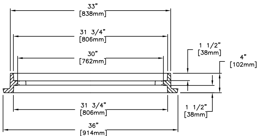
FRAME SECTION
