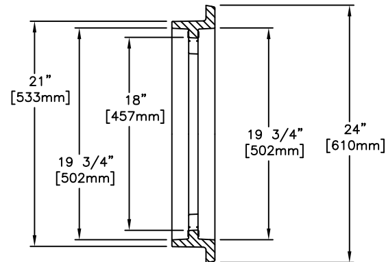
FRAME SECTION
