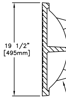
COVER SECTION
