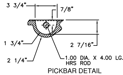
PICKBAR DETAIL
