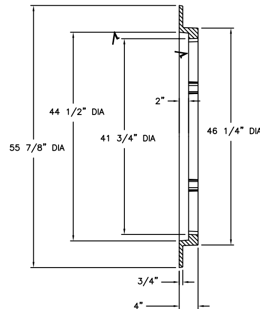
RING SECTION
