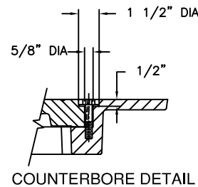
COUNTERBORE DETAIL
