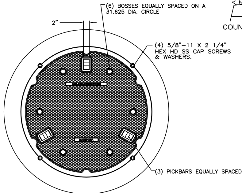
COVER BACK
