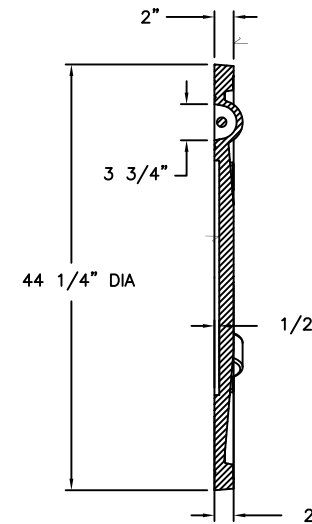
COVER SECTION
