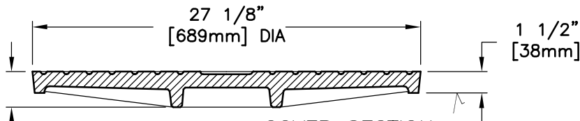
COVER SECTION
