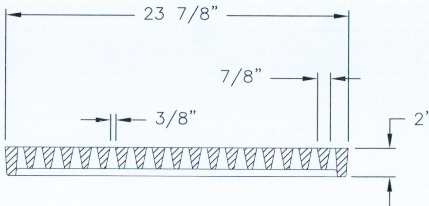
SECTION VIEW
