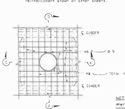
PART PLAN DECK ACCESS OPENING DETAIL U43
