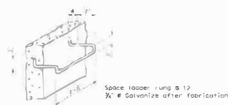
BAR STEP LADDER RUNG DETAILS DETAIL U44
