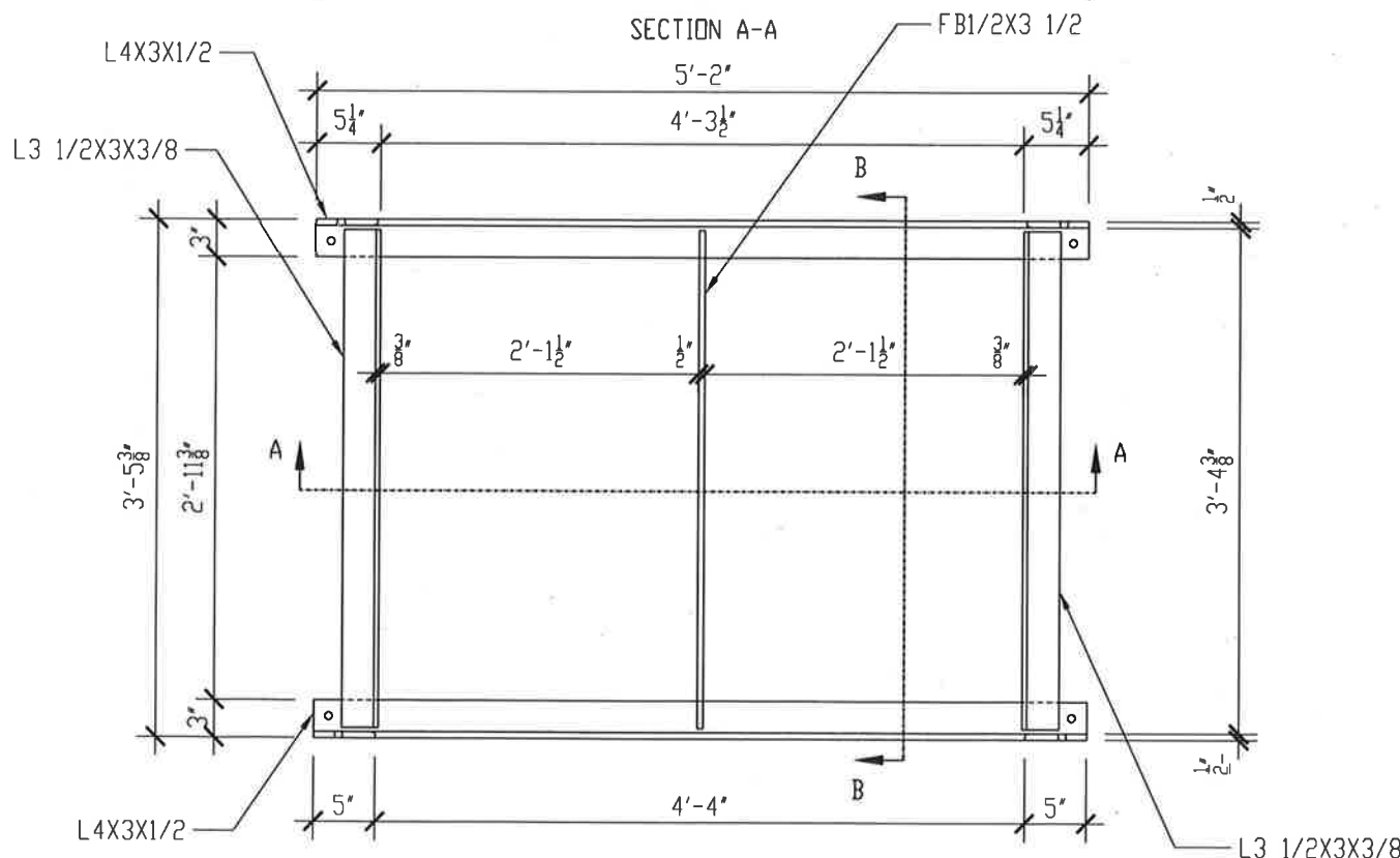
APWA 305 2 GRATES
