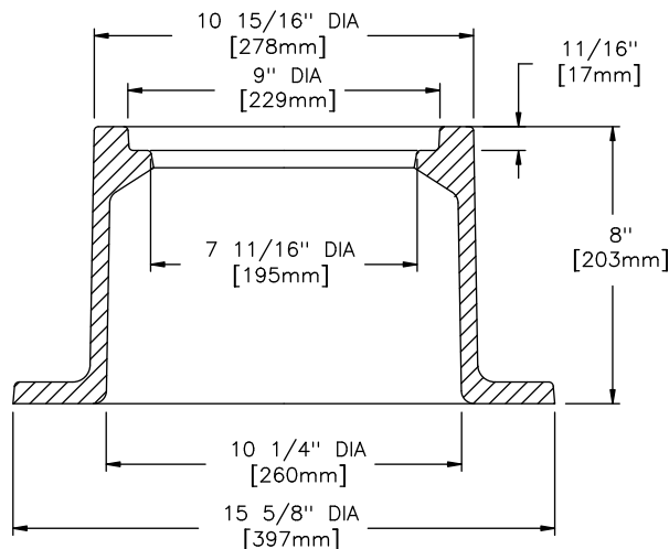
FRAME SECTION
