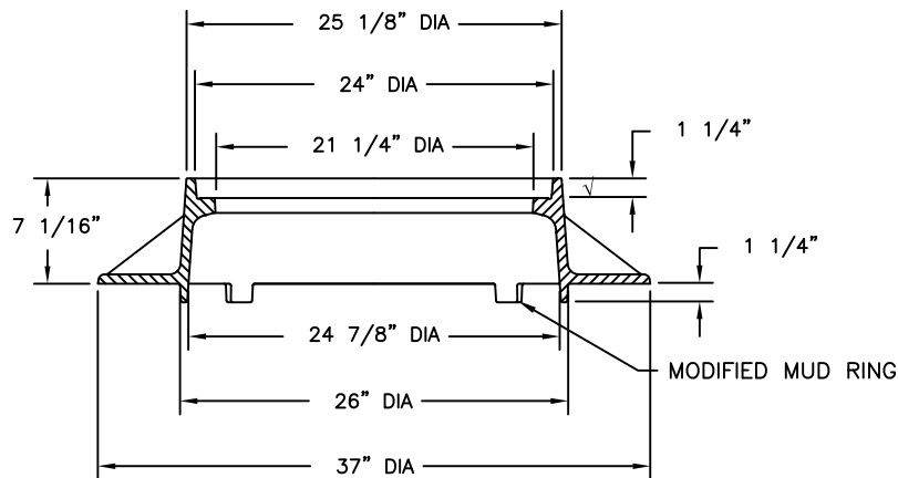
FRAME SECTION
