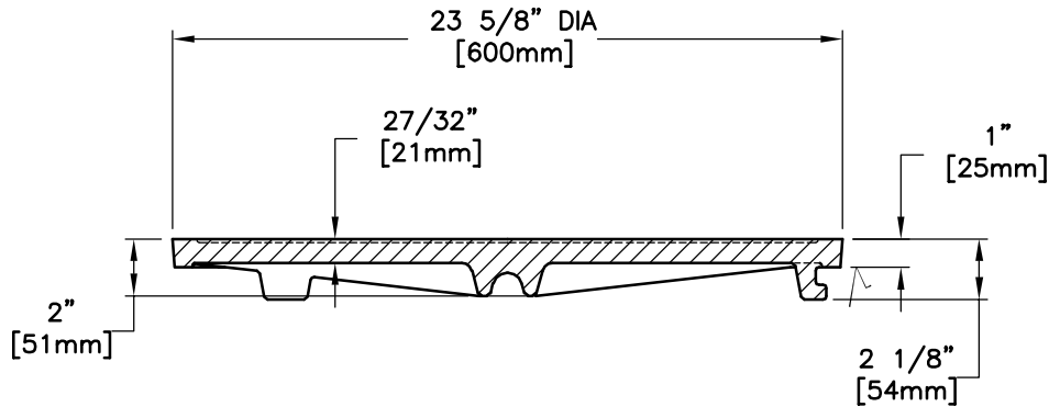
COVER SECTION
