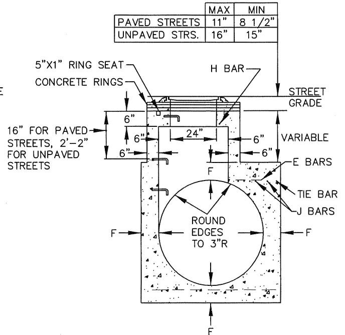
DETAIL M SEE NOTE ⑤
