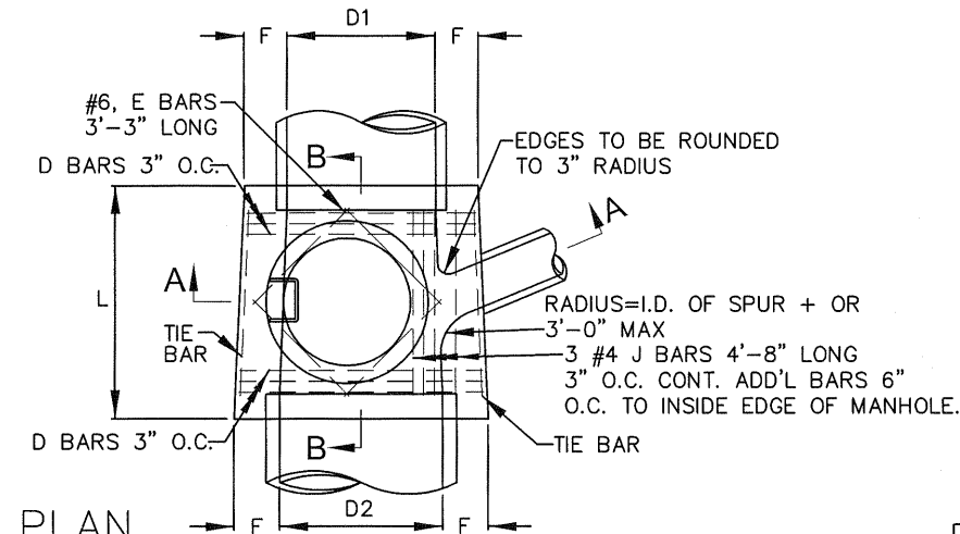
PLAN (SHAFT NOT SHOWN)
