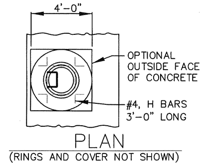
PLAN (RINGS AND COVER NOT SHOWN)
