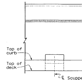
VIEW B-B
