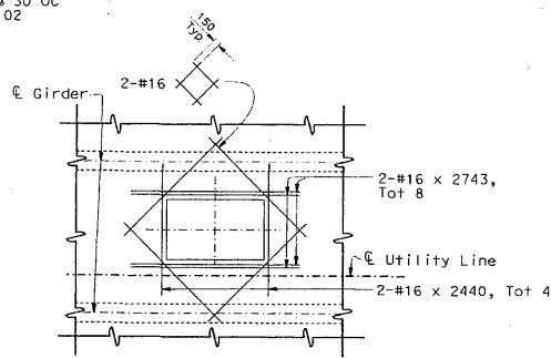
PLAN (SOFFIT GRATE OPENING) No Scale
