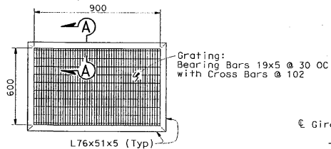
GRATE PLAN No Scale
