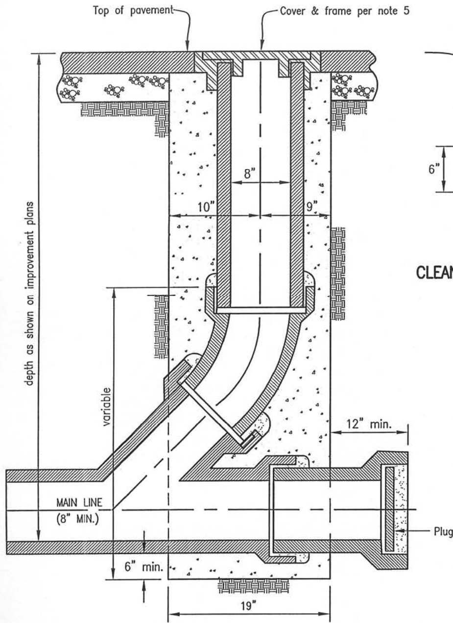
CLEAN-OUT FOR PAVED AREAS
