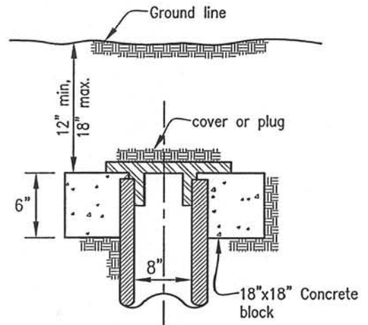
CLEAN-OUT FOR UNPAVED AREAS
