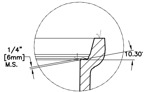
MACHINE DETAIL
