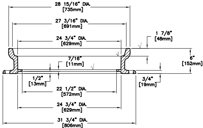
FRAME SECTION
