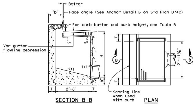
TYPE GO
