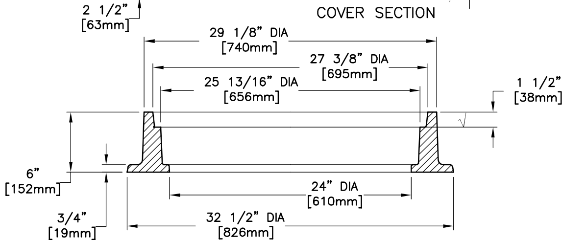
RING SECTION
