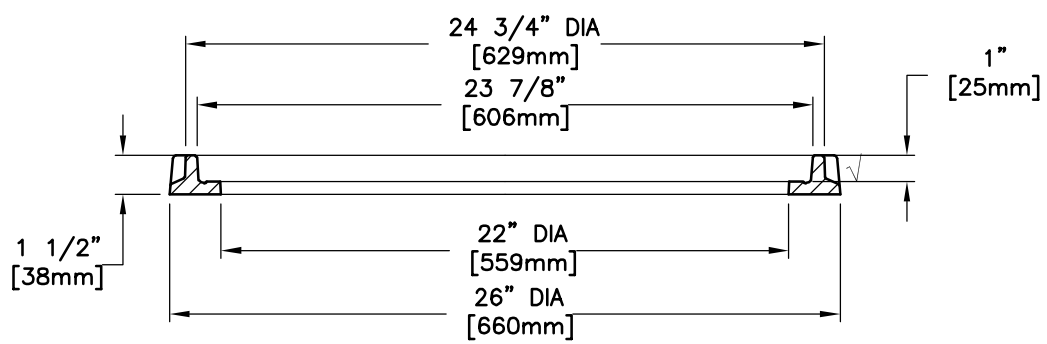
FRAME SECTION
