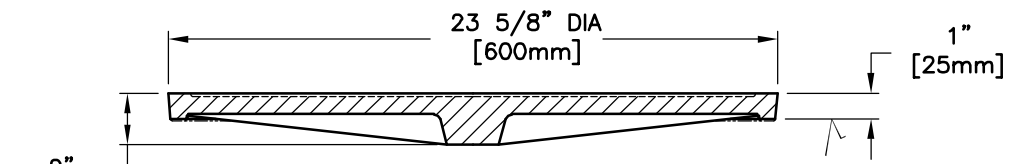
COVER SECTION
