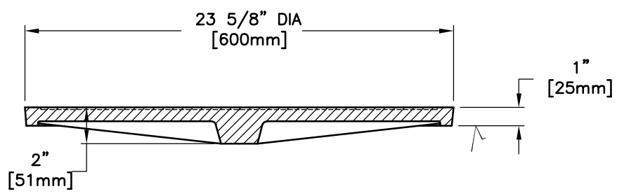
COVER SECTION
