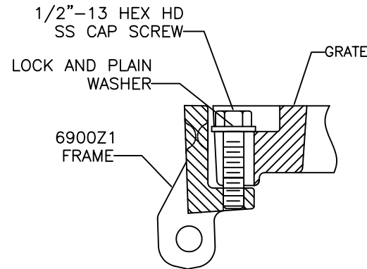
BOLT DETAIL
