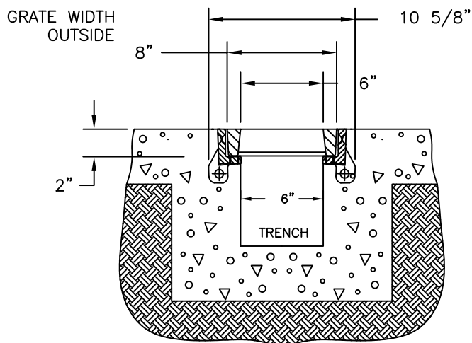
SECTION
