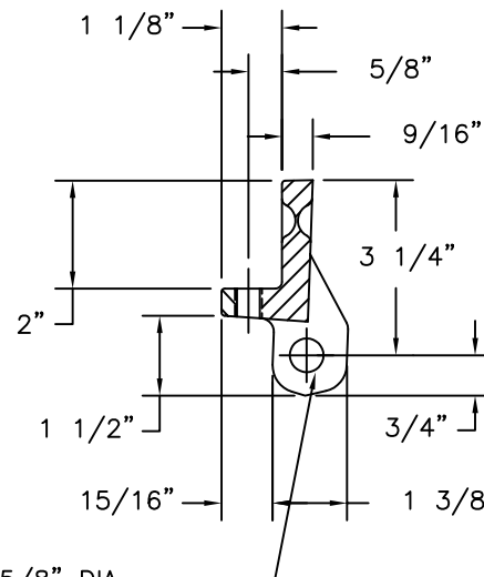
FRAME DETAIL
