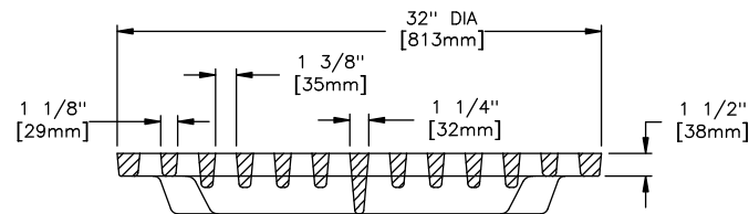
GRATE SECTION
