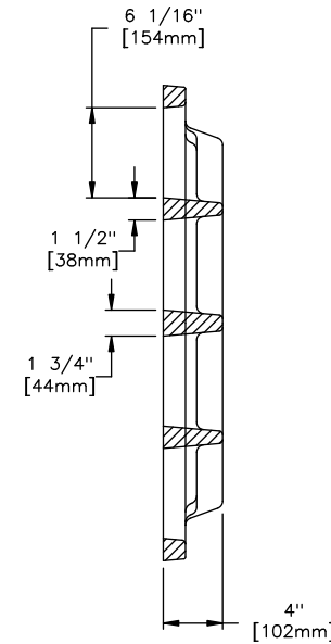
GRATE SECTION
