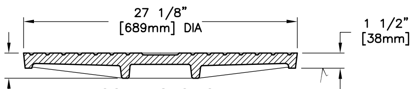
COVER SECTION
