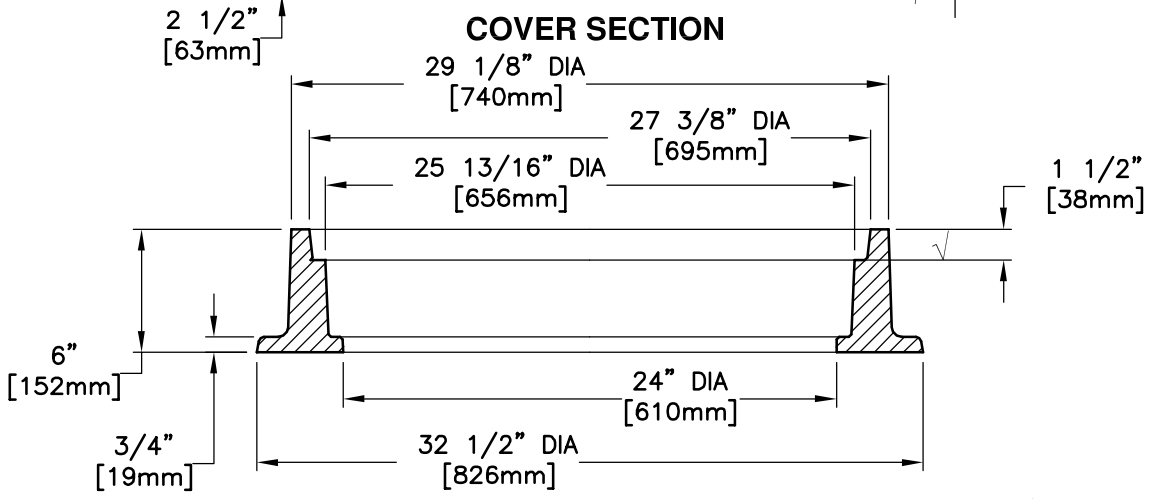
RING SECTION
