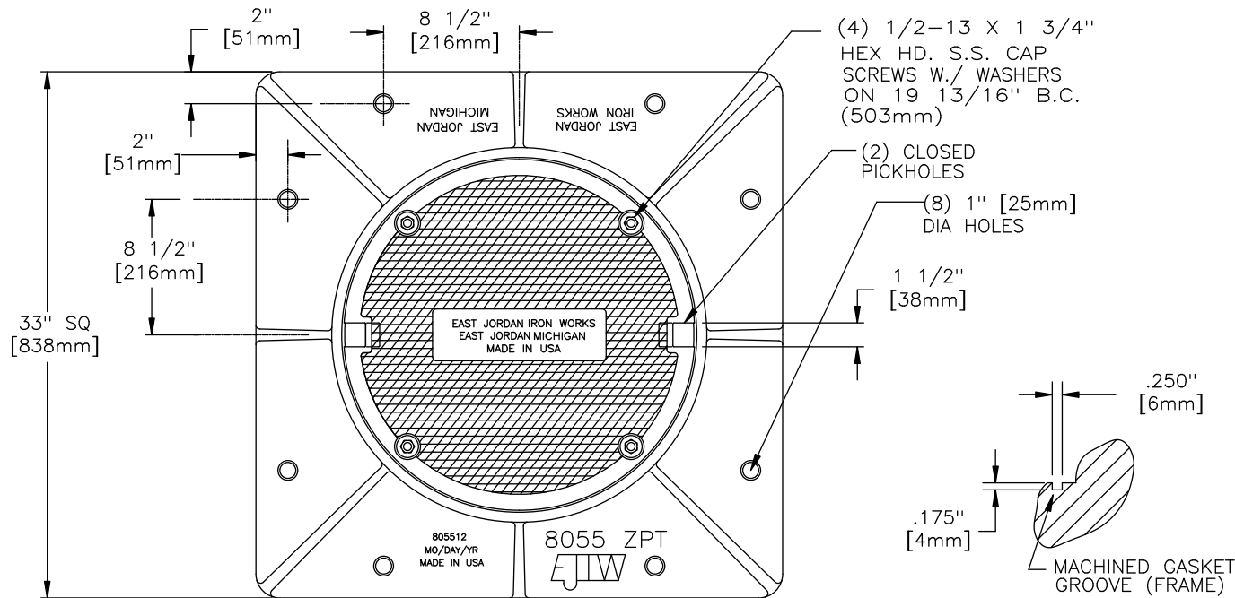
GROOVE DETAIL
