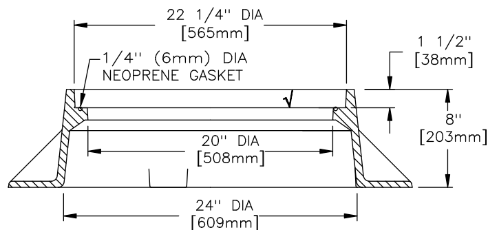
FRAME SECTION
