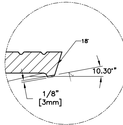
MACHINE DETAIL
